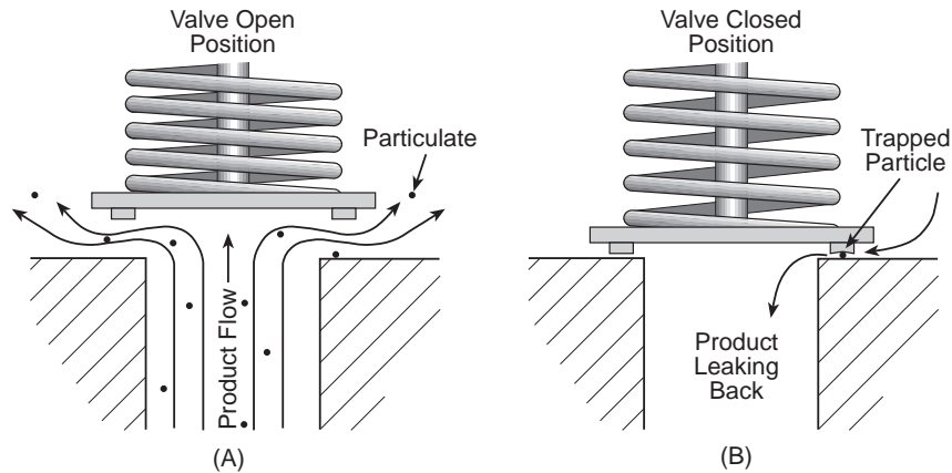
Figure 16 - Diagram of a Leaking Check Valve
